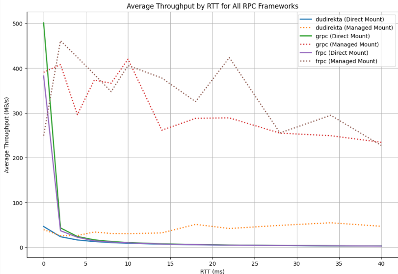
Figure 23: Average throughput by RTT for Dudirekta, gRPC and FRPC for managed and direct mount configurations.
